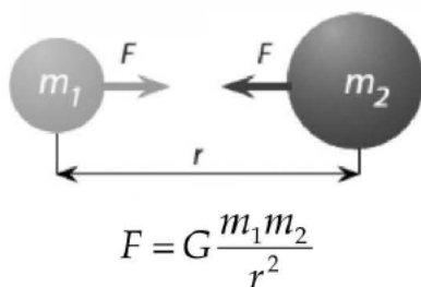
Fig 6.1 Newton's Law of Universal Gravitation
