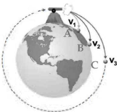
Fig 6.8 A cannon ball launched from high mountain
