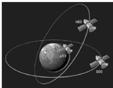
Fig 6.7 Motion of satellites in different orbits
